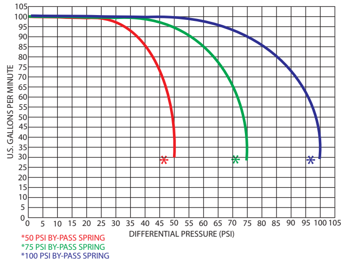
PUMP CURVE DATA
