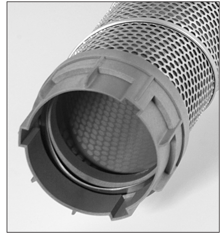
Open endcap with bayonet mount
